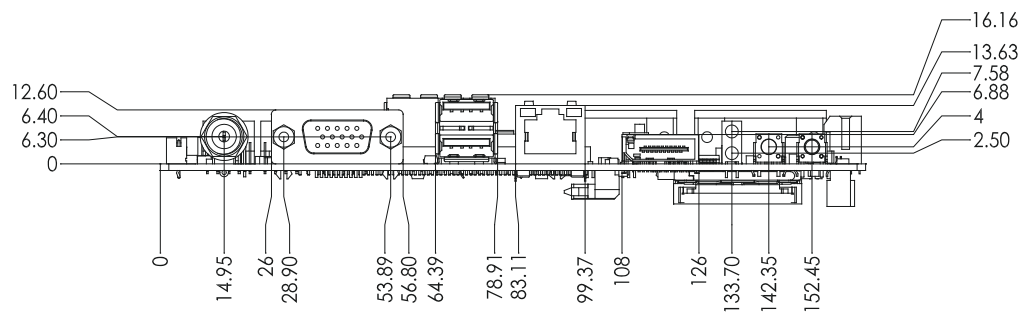
Figure 1.7 MIOe-DB2100 Mechanical Drawing (Front I/O, with optional DC Jack)
