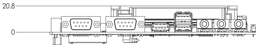
Figure 1.10 MIO-3260 + MIOe-DB2100 Height Dimension (With optional heatspreader)
