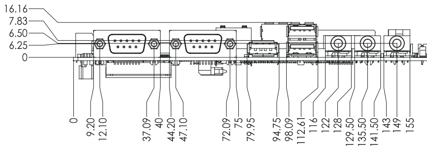
Figure 1.8 MIOe-DB2100 Mechanical Drawing (Rear I/O)
