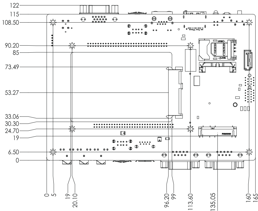
Figure 1.4 MIOe-DB2100 Mechanical Drawing (Bottom Side)
