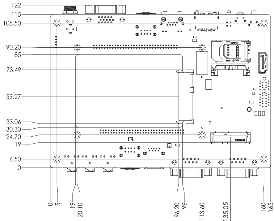
Figure 1.5 MIOe-DB2100 Mechanical Drawing (Bottom Side, with optional DC Jack)
