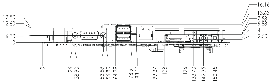
Figure 1.6 MIOe-DB2100 Mechanical Drawing (Front I/O)
