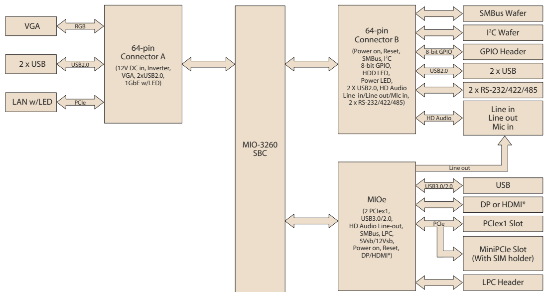
Figure 1.1 Block Diagram
