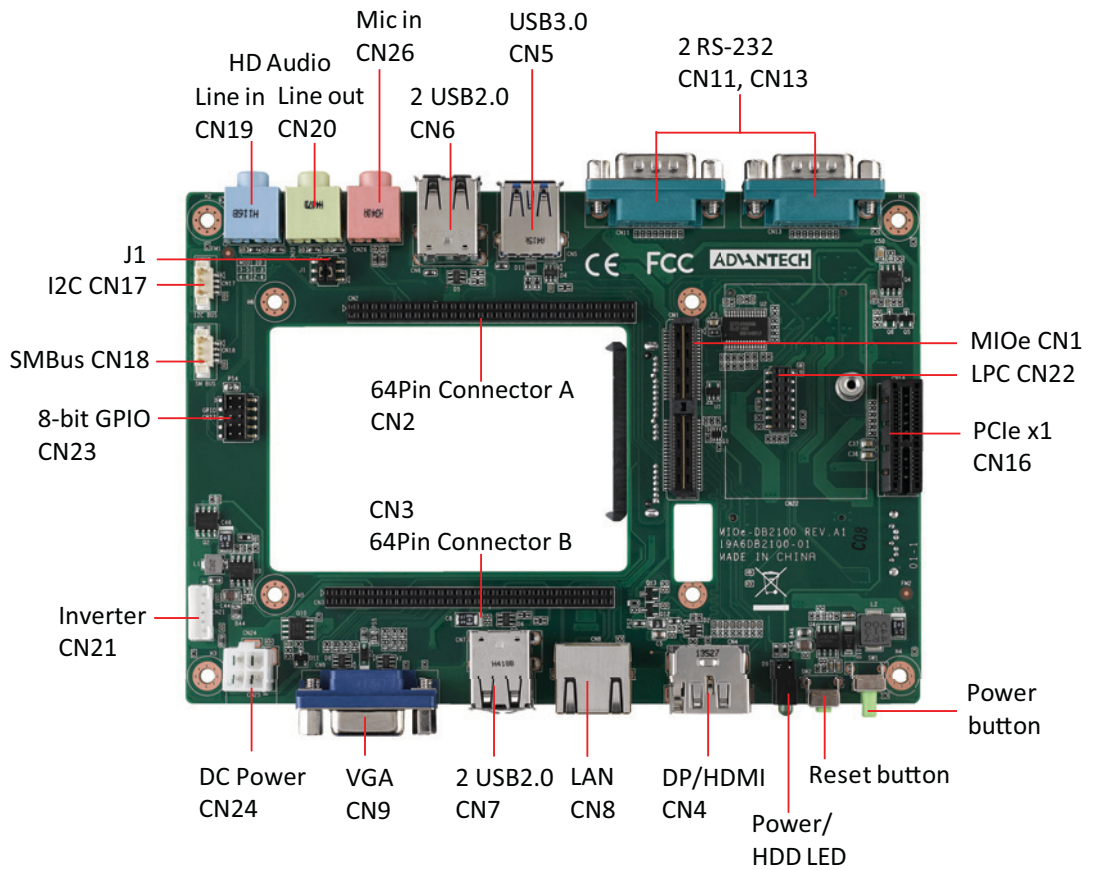
Figure 2.1 Jumper and Connector layout (Top side)
