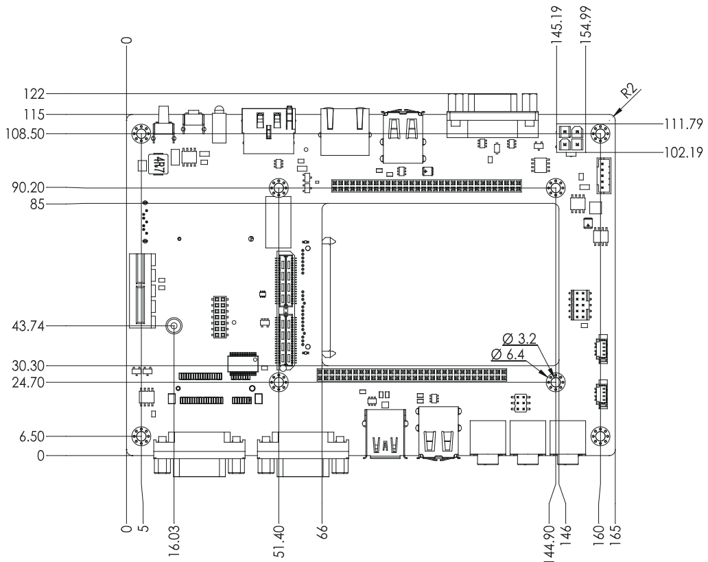
Figure 1.2 MIOe-DB2100 Mechanical Drawing (Top Side)
