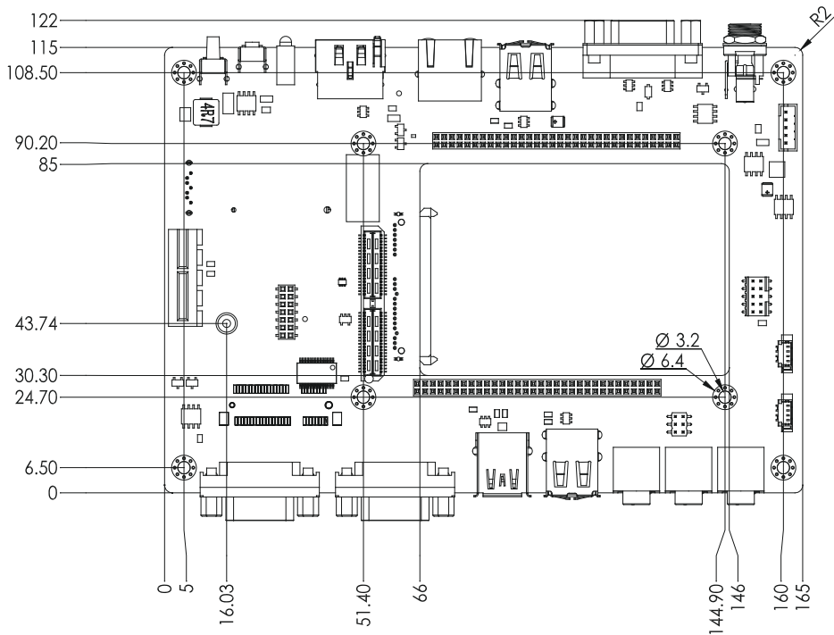
Figure 1.3 MIOe-DB2100 Mechanical Drawing (Top Side, with optional DC Jack)
