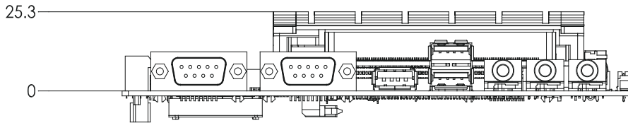
Figure 1.9 MIO-3260 + MIOe-DB2100 Height Dimension (With standard heatsink)
