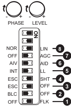
Figure 7. Switch Settings (Defaults)
