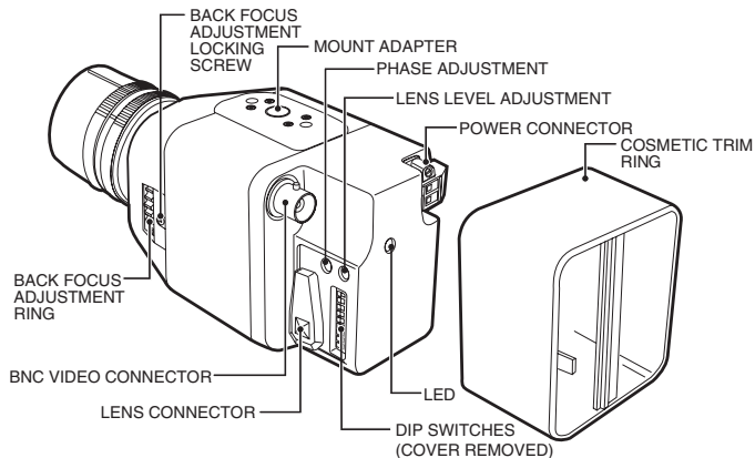
Figure 1. Camera Layout
