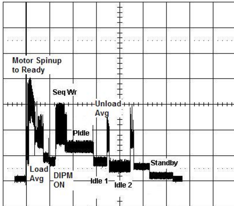
Figure 1 Typical 5V Startup and Operation Current Profile
