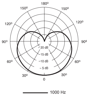
1000 Hz Polar Pattern Measured at 1000 Hz
