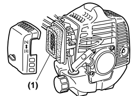
(1) Air filter
