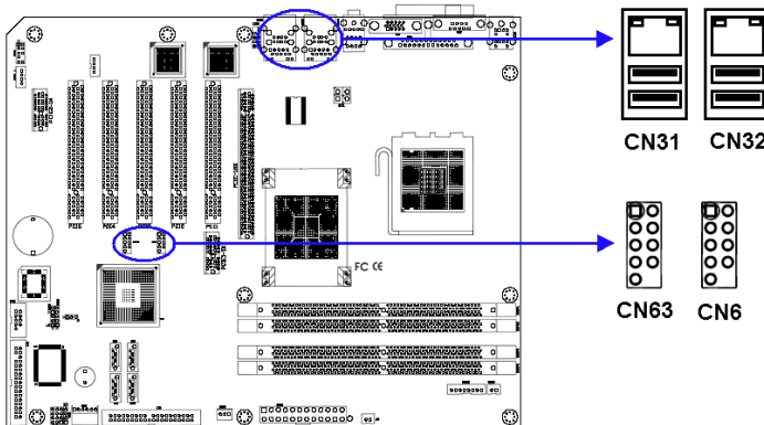
Figure 2.1: USB Ports
