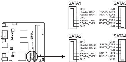
AT3IONT-I SERIES SATA connectors
