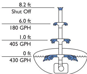
Average Performance
