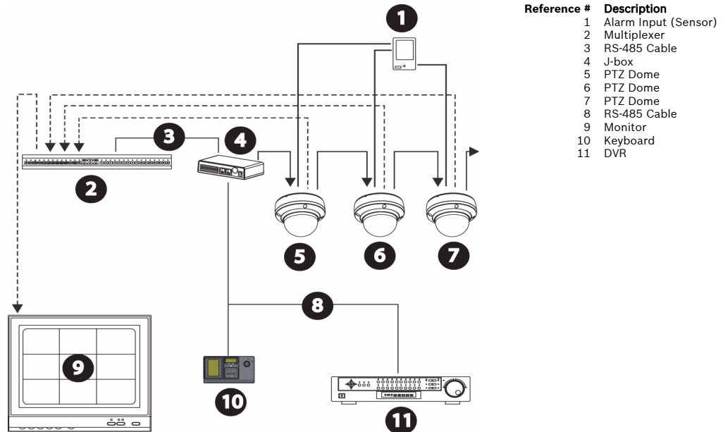
Fig. 2.1 System Configuration
