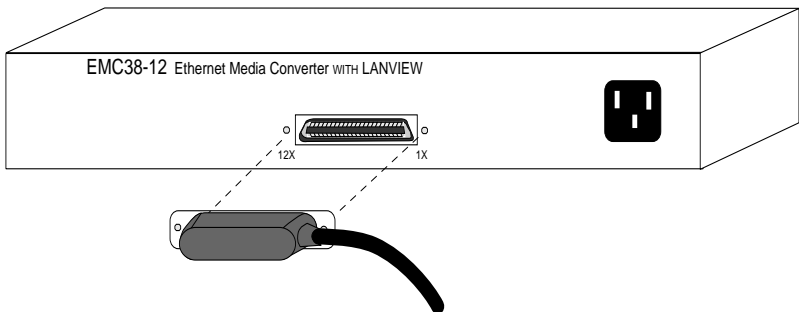
Figure 3-1. EMC38-12
