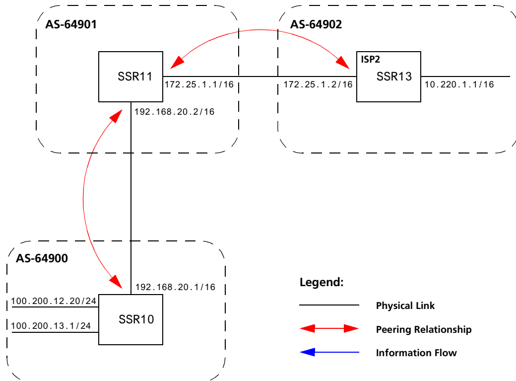
Figure 6. Sample BGP Configuration (Well-Known Community)
