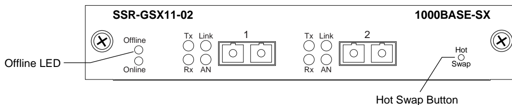
Figure 14. Location of Offline LED and Hot Swap button on a 1000 BASE-SX line card
