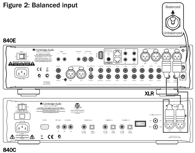
Figure 2: Balanced input
