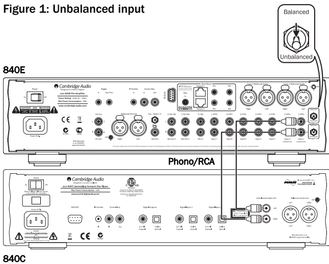
Figure 1: Unbalanced input
