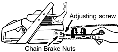
Adjusting Screw - 1/4 Turn
